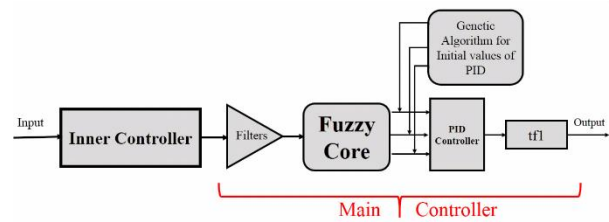
Figure7: Controller 1 scheme
